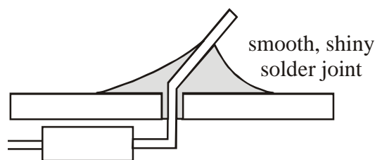
Figure 15.8 A Successful Solder Joint
